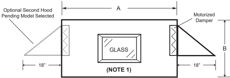
Elevator Vent
