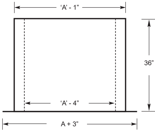
Roof Curb
